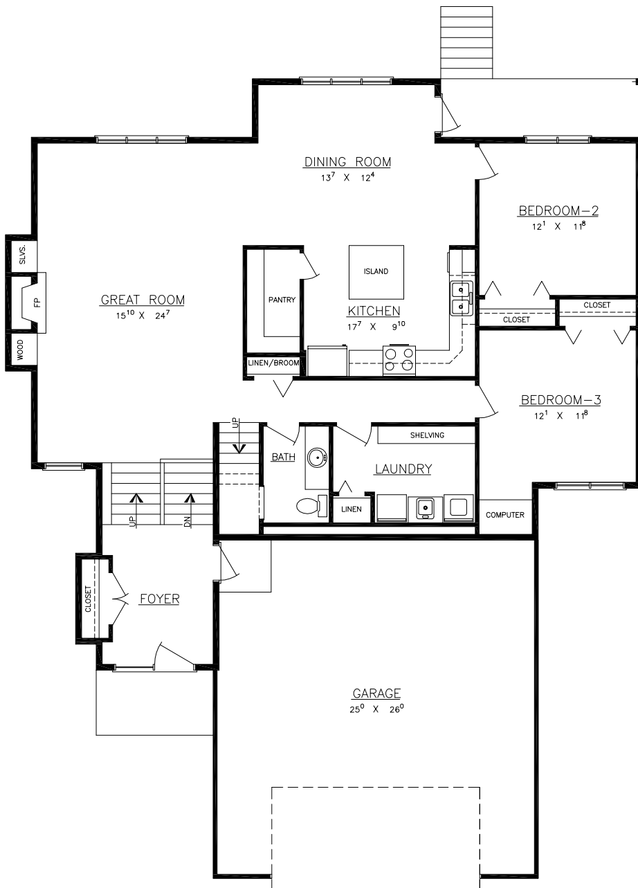
MAIN LEVEL
